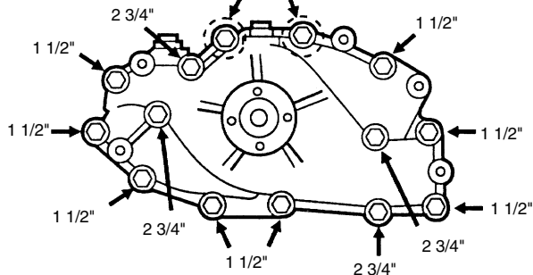
Water Pump Mounting Bolt Lengths and Locations
