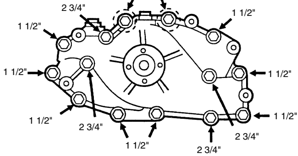
Water Pump Mounting Bolt Lengths and Locations
