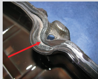
Split gasket caused by over torquing
