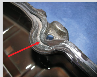
Split gasket caused by over-torquing
