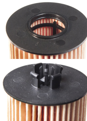
Our updated end cap with new bypass valve
